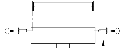
4. Tie up side screws
