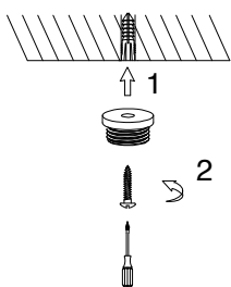
3. Tie up the screws into the anchors
