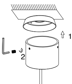
7. Apply the lid by tiding up the screws
